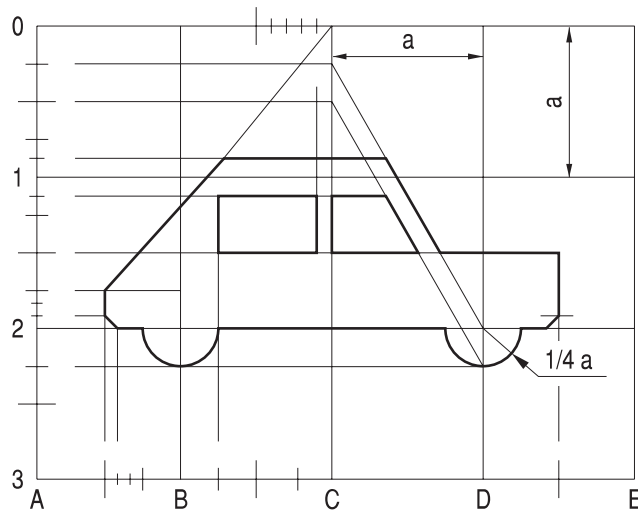
Rys. 9.1.38. Symbol samochodu
